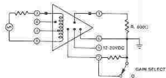
FIGURE 2. 1588C CONNECTION DIAGRAM
