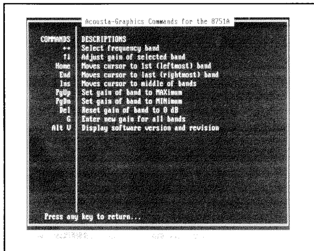
Figure 6 Help Screen
