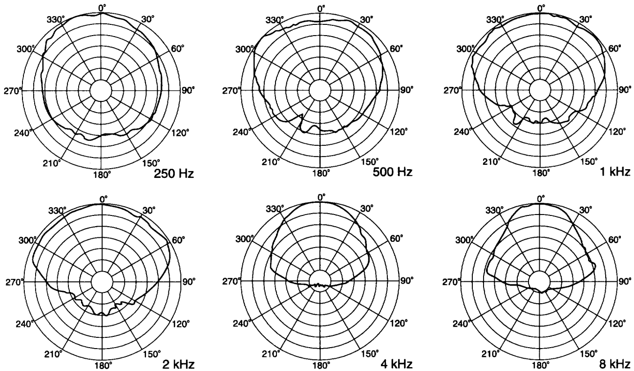
Figure 1—Polar Response
