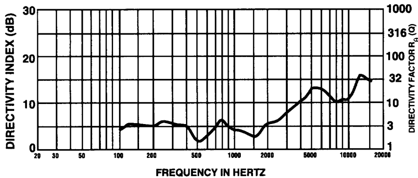
Figure 5 Directivity
