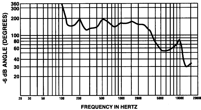
Figure 4 Beamwidth
