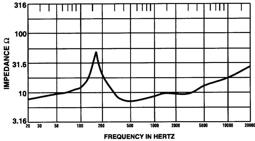
Figure 3 Impedance
