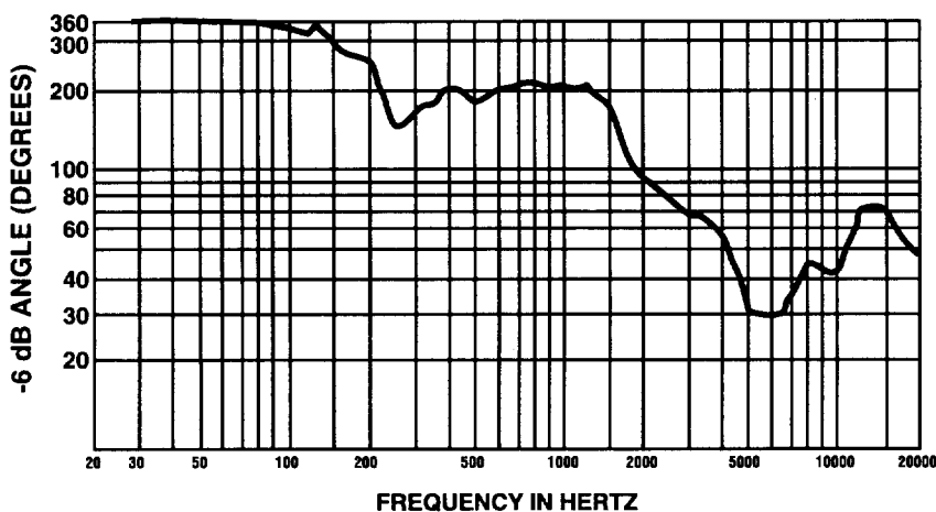
Figure 4 Beamwidth
