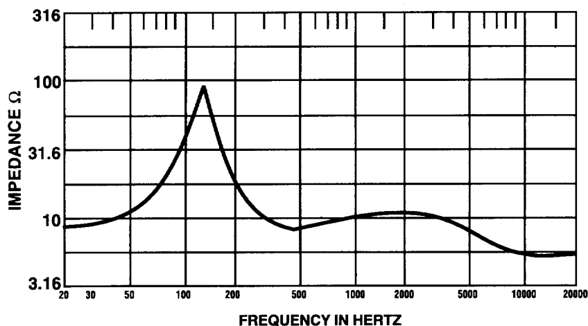
Figure 3 Impedance
