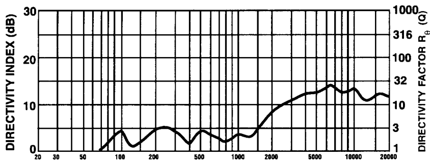
Figure 5 Directivity
