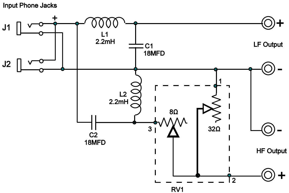
N809-8A Crossover Network
