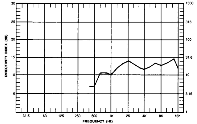
Figure 9. Q and Directivity Index
