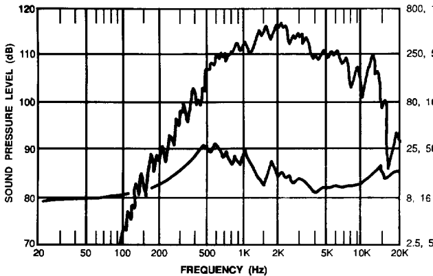
Figure 1. Frequency Response and Magnitude of Impedance with 299-A Driver (See Note 2)
