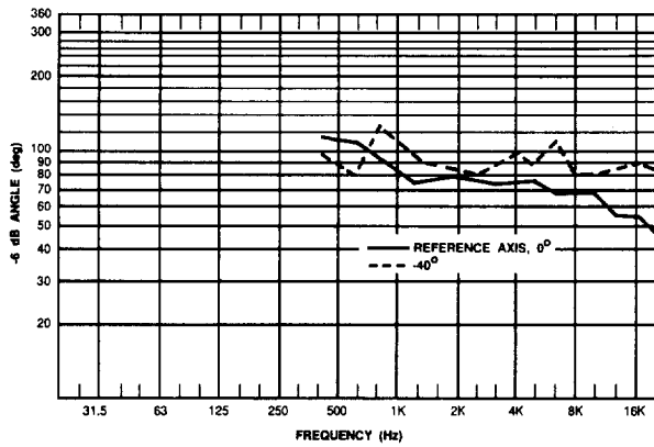
Figure 8. Dispersion Angle
