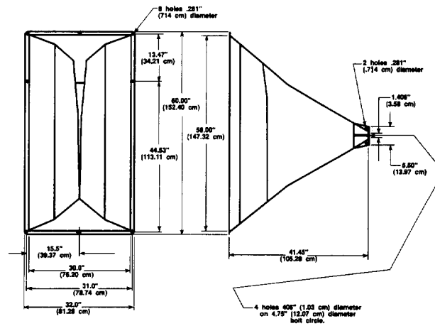
Figure 10. Mounting Information and Dimensions
