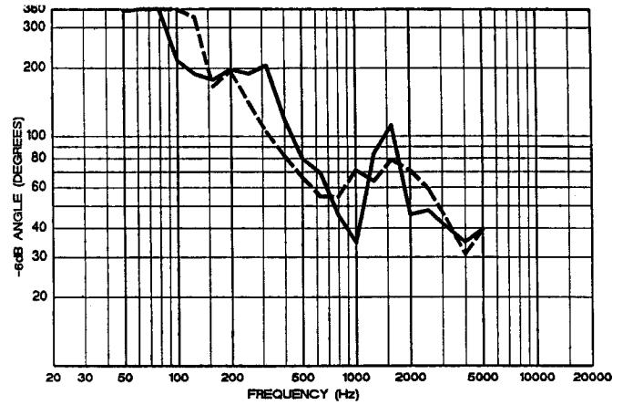
Figure 3. Dispersion Angle
