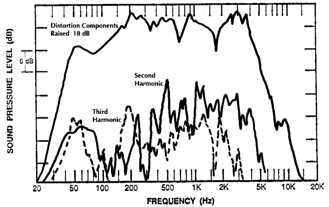
Figure 7. Harmonic Distortion at 0.1 Rated Power
