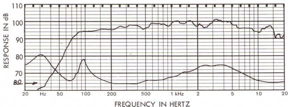
Figure 1. Frequency Response of Typical 937 System
